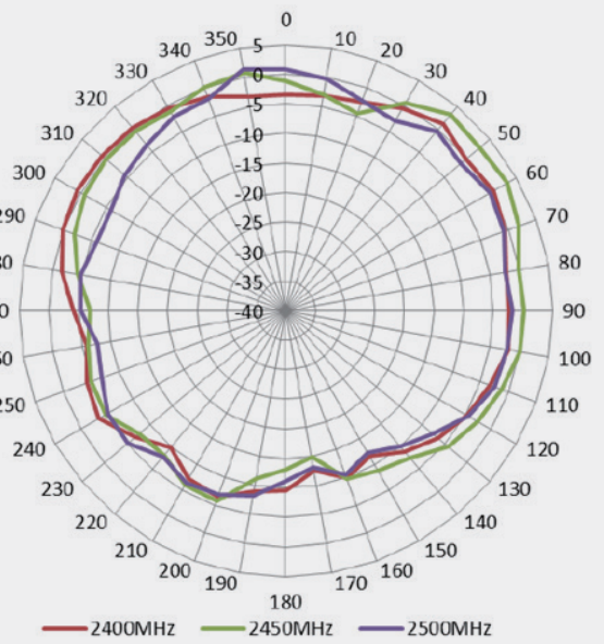
2.4G (PHI=90)
