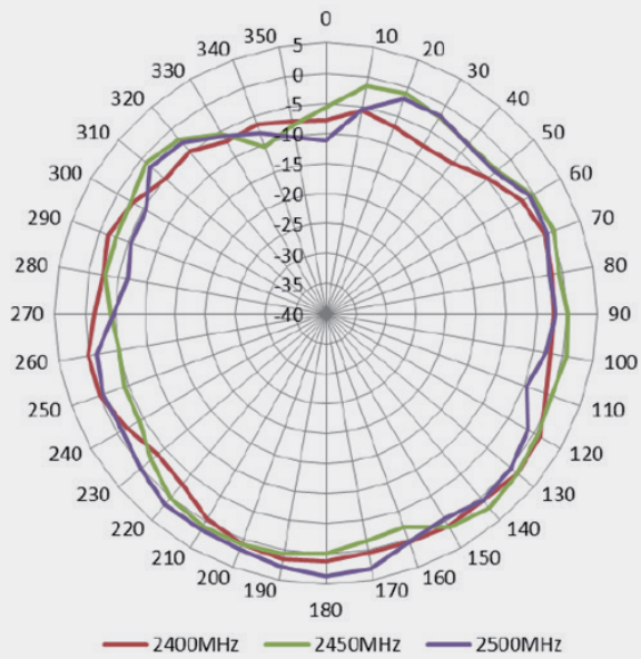
2.4G (PHI=0)
