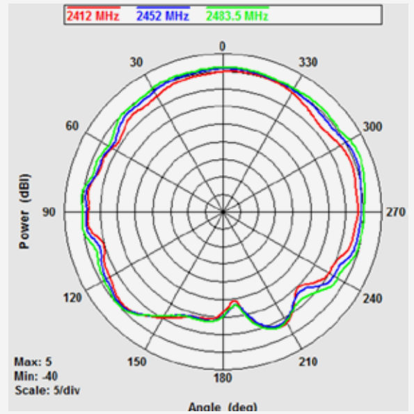
2.4G (PHI=90)
